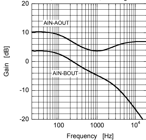
Gain vs Frequency (ViVA)
