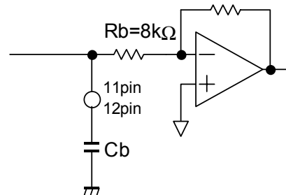
Smoothing circuit of Boost
