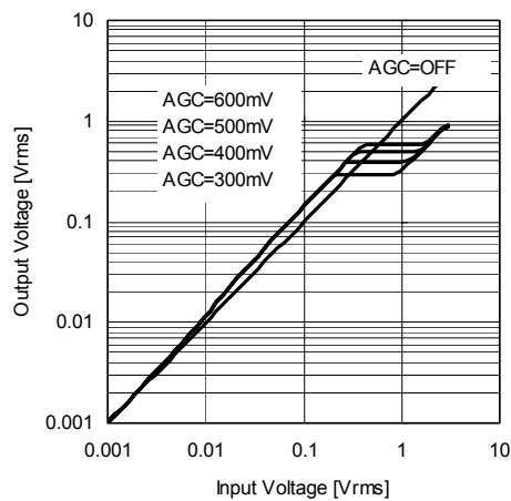
AGC Output Voltage vs. Input Voltage Ta=25°C, V+=9V, R i =47kΩ, Vin(A+Bch), f=1kHz, Vout(Ach), BW=400Hz-30kHz, VOL=0dB, BAL=0dB, BASS=TREB=0dB, BBE=OFF, Surround=OFF
