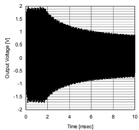
AGC Attack Time Response Ta=25°C, V+=9V, R i =47kΩ, Vin(A+Bch), f=20kHz, Vout(Ach), BW=400Hz-30kHz, VOL=0dB, BAL=0dB, AGC=300mV, BASS=TREB=0dB, BBE=OFF, Surround=OFF
