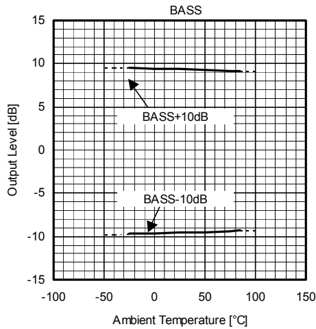
Tone Control Output Level vs. Ambient Temperature V_{+}=7V V_{-}=-7V V_{dd}=5V
