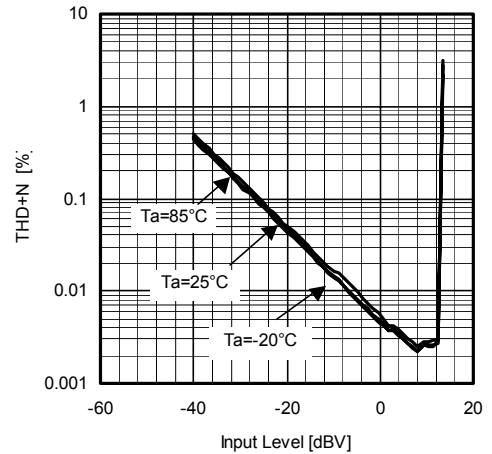
Volume THD+N vs. Input Level 0dB Setting f=1kHz
