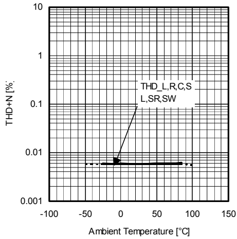
Volume THD+N vs. Ambient Temperature V_{+}=7V V_{-}=-7V V_{dd}=5V , 0dB Setting
