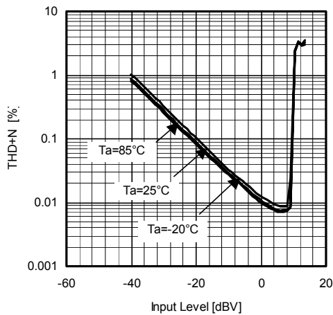
Tone Control THD+N vs. Input Level Flat (0dB) Setting f=1kHz
