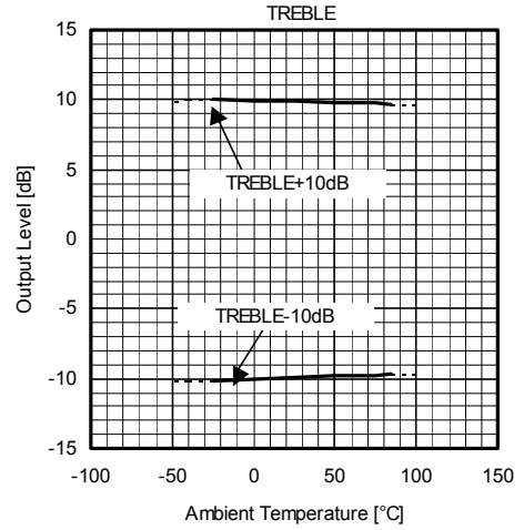
Tone Control Output Level vs. Ambient Temperature V_{+}=7V V_{-}=-7V V_{dd}=5V
