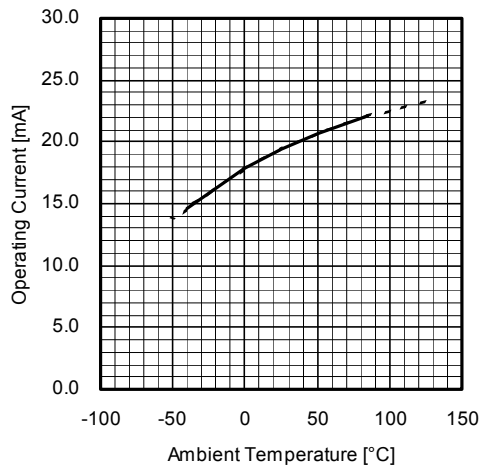
Operating Current vs. Ambient Temperature IEE V+=7V V-=-7V
