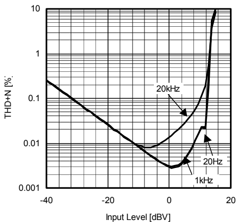
Volume THD+N vs. Input Level INPUT:LAIN OUTPUT:L.OUT TONEon BW=10Hz-80kHz Ta=25°C
