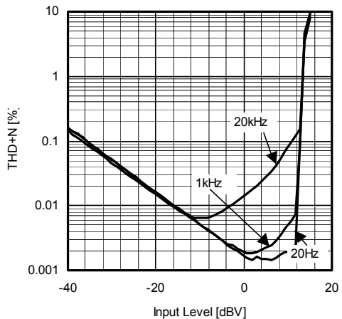
Volume THD+N vs. Input Level INPUT:L1IN OUTPUT:REC1L V+=7V V-=-7V RL=10kΩ BW=10Hz-80kHz Ta=25°C
