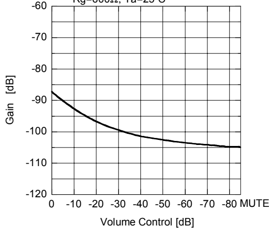
Output Noise vs Volume Control
