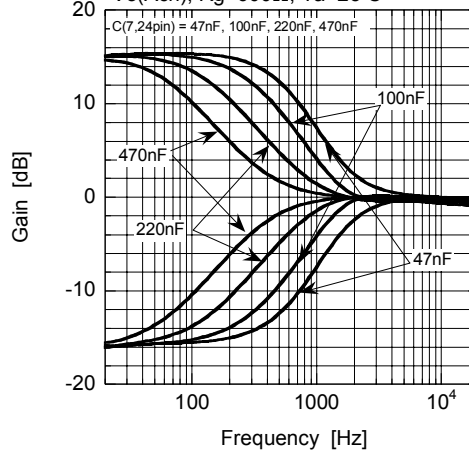
AGC Control
