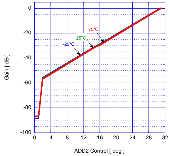
Gain vs ADD2 Control
