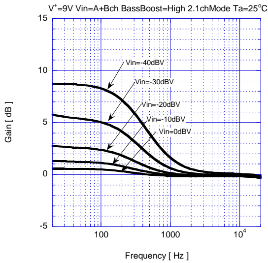
Gain vs Frequency (BB-AGCOUT, LPF)
