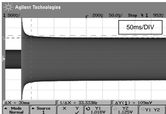
BB-AGC Attack Time
