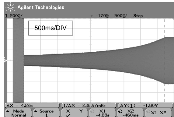
BB-AGC Recovery Time
