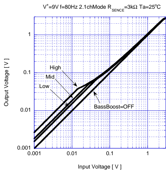
BassBoost AGC Characteristics (BPF)
