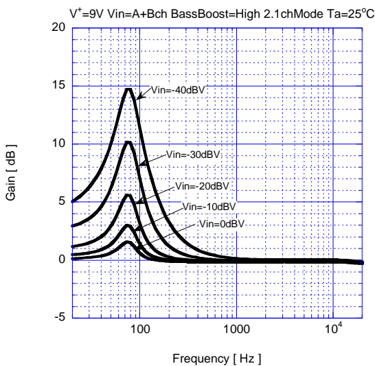
Gain vs Frequency (BB-AGCOUT, BPF)
