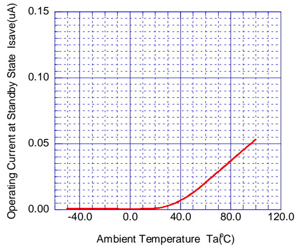
Operating Current at Standby State vs. Temperature
