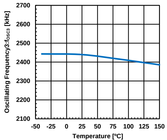
Oscillating Frequency vs. Temperature ( V+=12\text{V} , R_T=2.32\text{k}\Omega )
