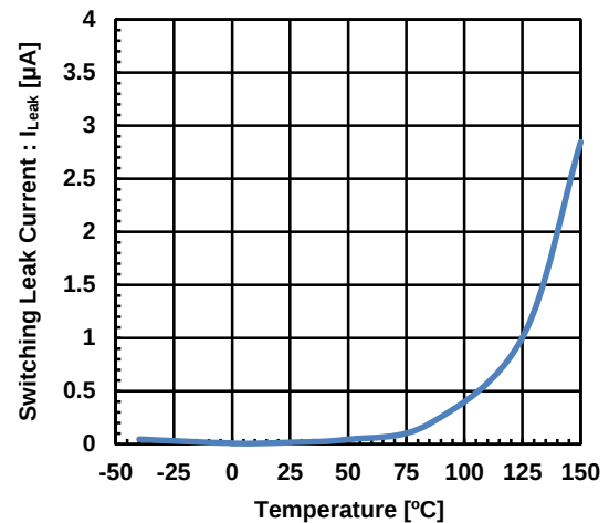
Switching Leak Current vs. Temperature ( V^+=12V , V_{EN}/V_{SYNC}=0V , V_{SW}=40V )
