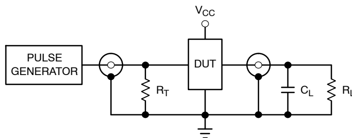
Figure 6. Test Circuit
