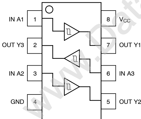
Figure 1. Pinout
