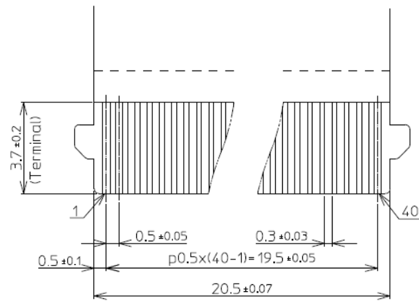
Adaptable socket : FH28-40S-0.5SH(05)
