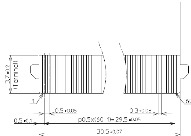
Adaptable socket : FH28-60S-0.5SH(05)
