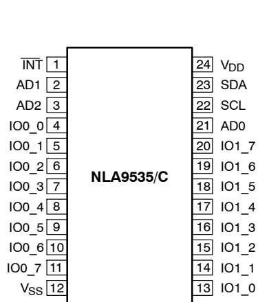
Figure 3. SOIC24 / TSSOP24
