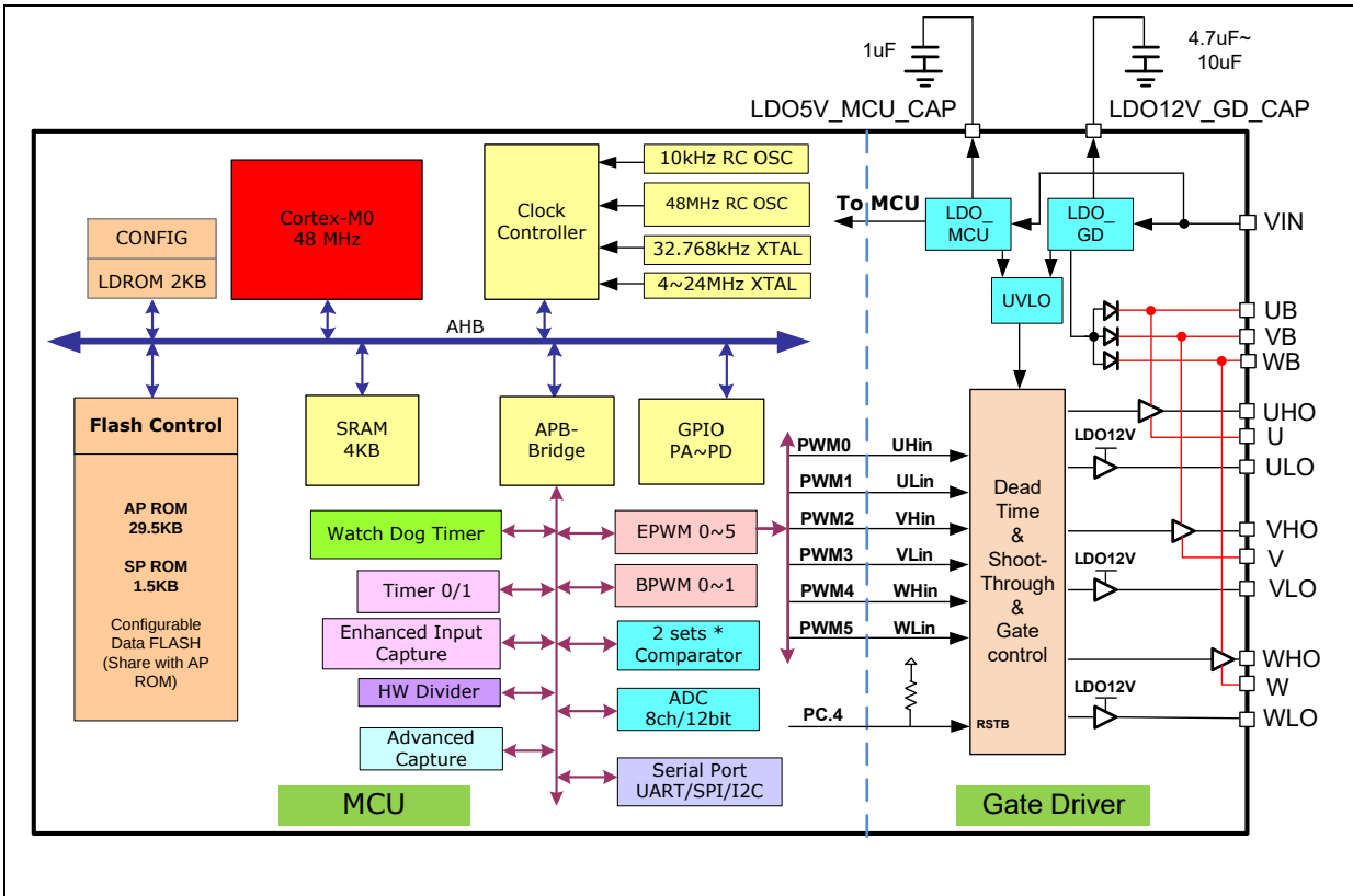
Figure 4.1-1 NM18107 Series Block Diagram
