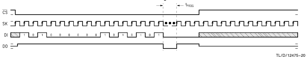
Write Timing
