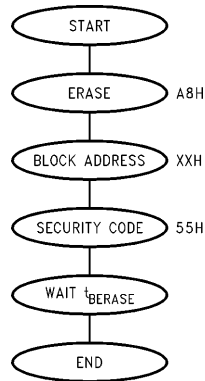
FIGURE 4. Block Erase Sequence
