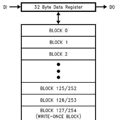
FIGURE 5. Device Organization
