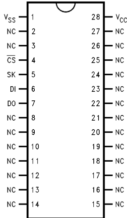
NM29A040M NM29A080M NS Package Number MA28A
