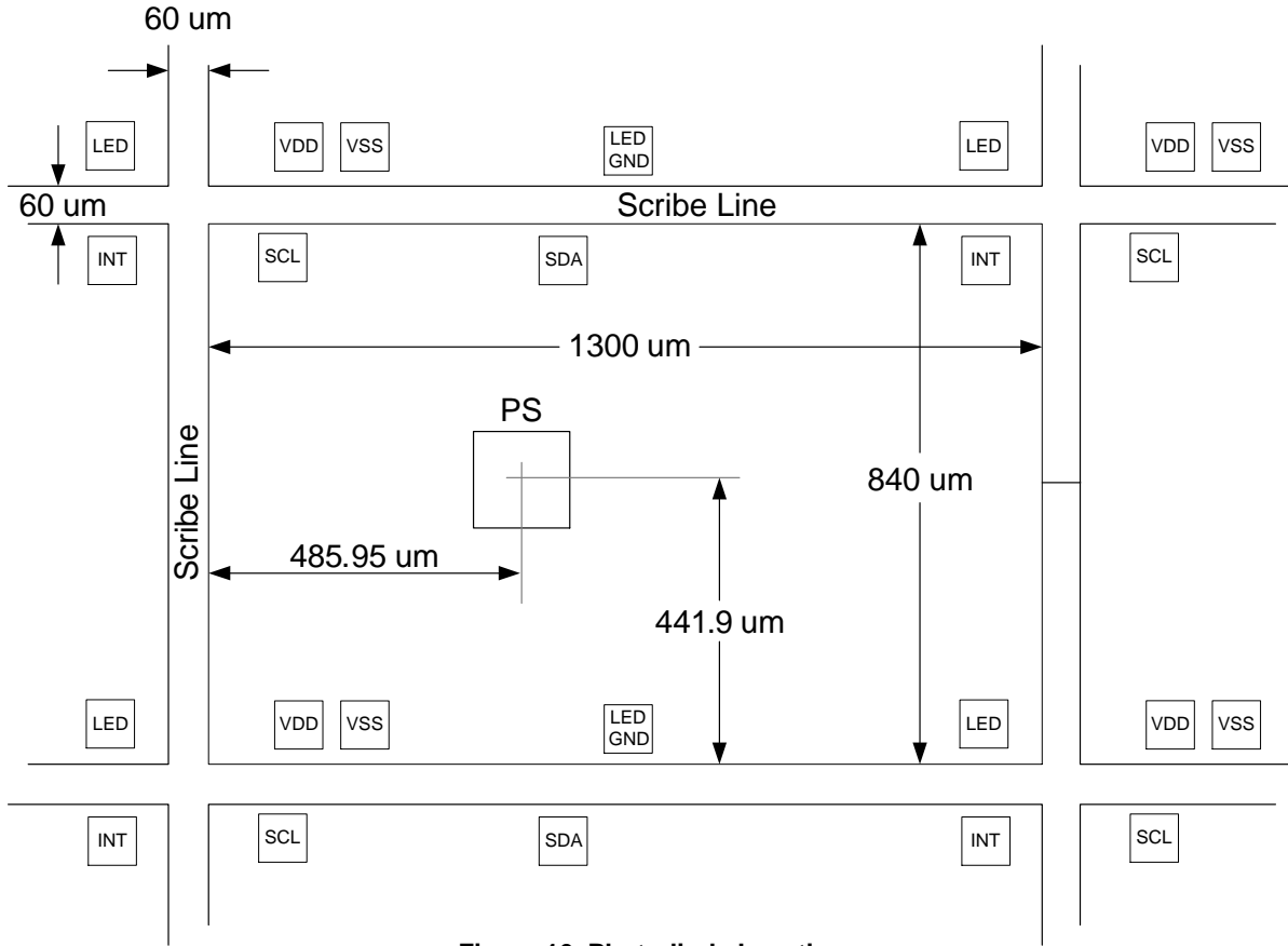
Figure 16. Photodiode Location
