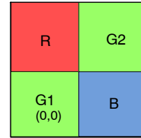
Figure 4. Color Filter Arrangement of Pixels
