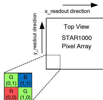
Figure 7. Bayer Pattern for STAR1000
