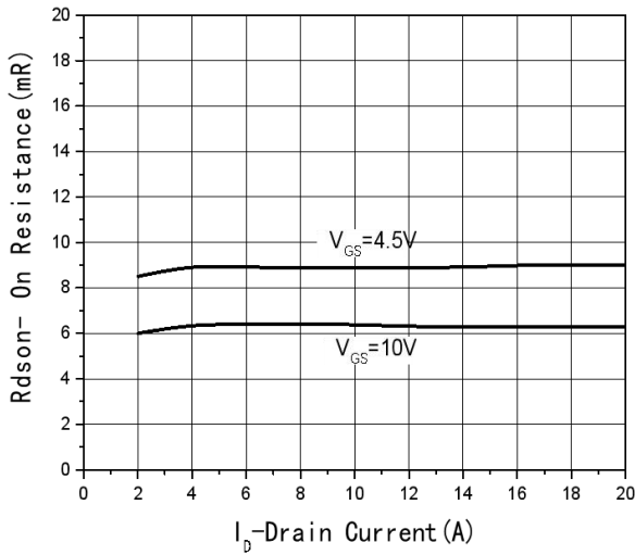
Fig3 Rdson-Drain current
