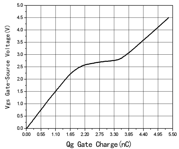
Fig6 Gate Charge
