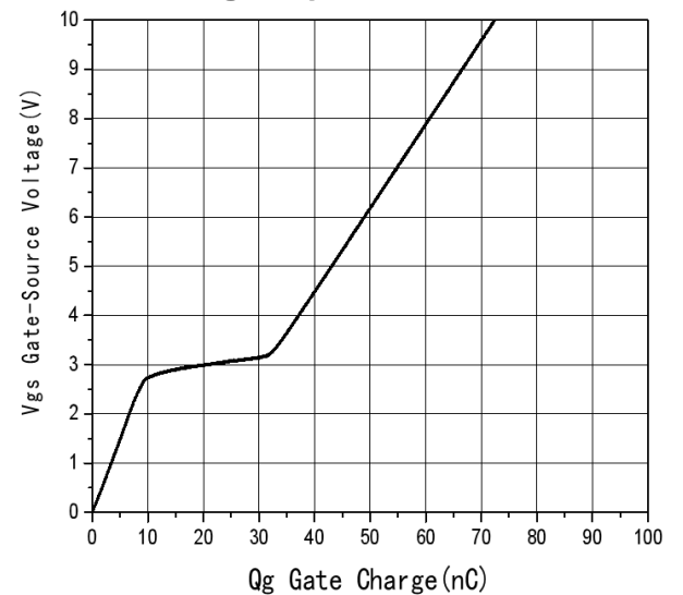
Fig6 Gate Charge
