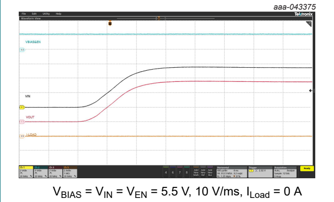
Fig. 9. Turn ON V IN
