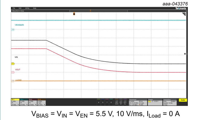
Fig. 10. Turn OFF V IN
