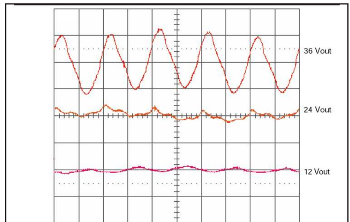
Figure 6: Output Voltage Ripple with 24V input and rated load current (50 mV/div). Load capacitance: 100μF electrolytic cap. Bandwidth: 20MHz. See Figure 4.
