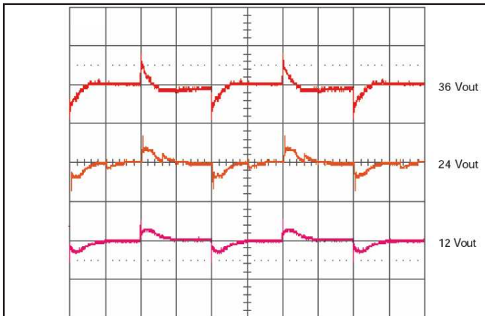
Figure 11: Output voltage response for 24V input; 12V, 24V, 36V output to step-change in load current (50-75-50% of I out max; di/dt=0.1A/µs). Load cap: 100µF, 100mΩ ESR tant, Ch 1-3: Vout (2V/div);(5ms/div).
