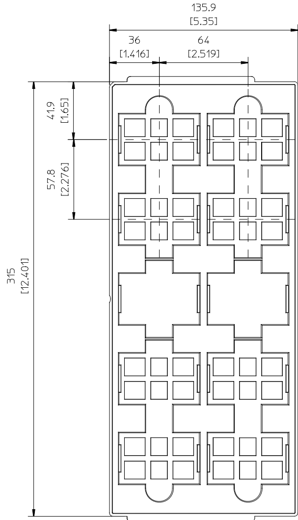
JEDEC standard tray for 2x5 = 10 products. All dimensions in mm [inch] Tolerances: X.x ±0.26 [0.01], X.xx ±0.13 [0.005] Note: pick up positions refer to center of pocket. See mechanical drawing for exact location on product.
