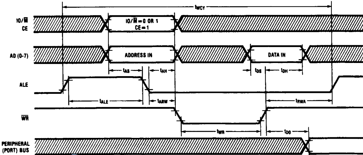
Write Cycle (Write to Port)
