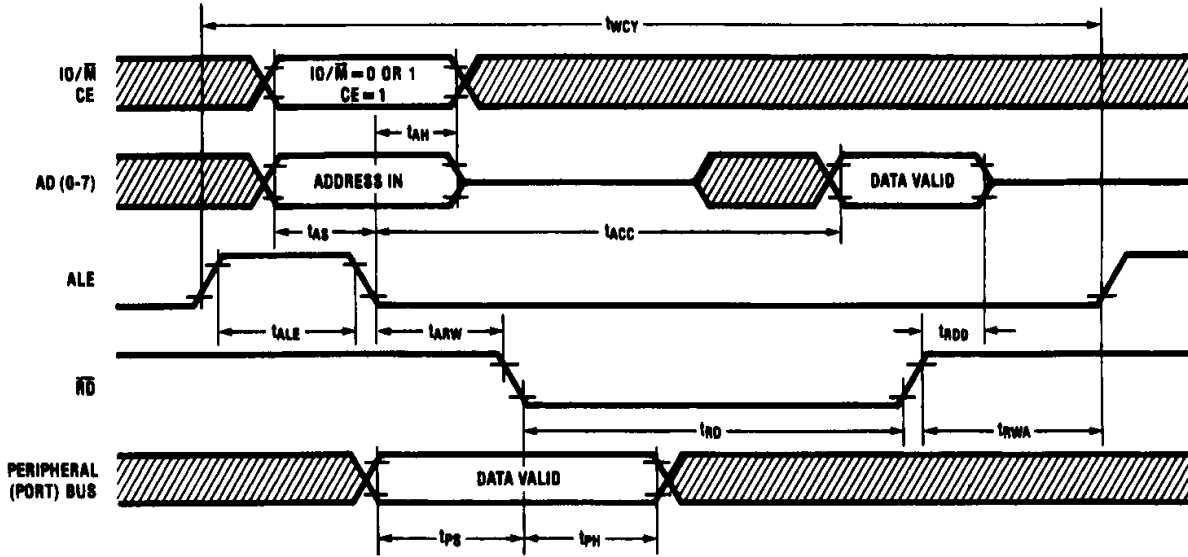
Read Cycle (Read from Port)
