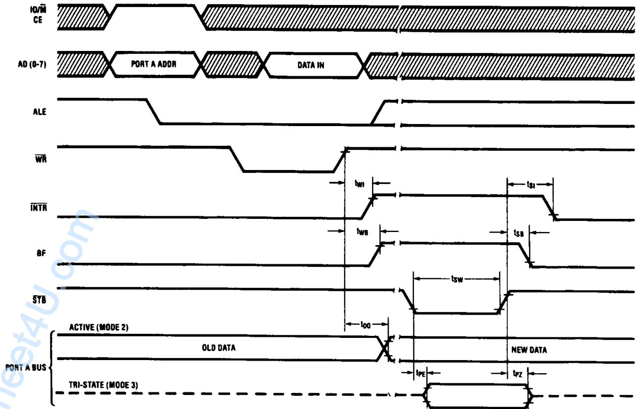
Strobed Mode Output
