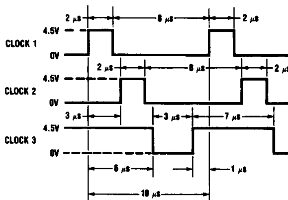
Input Clocks
