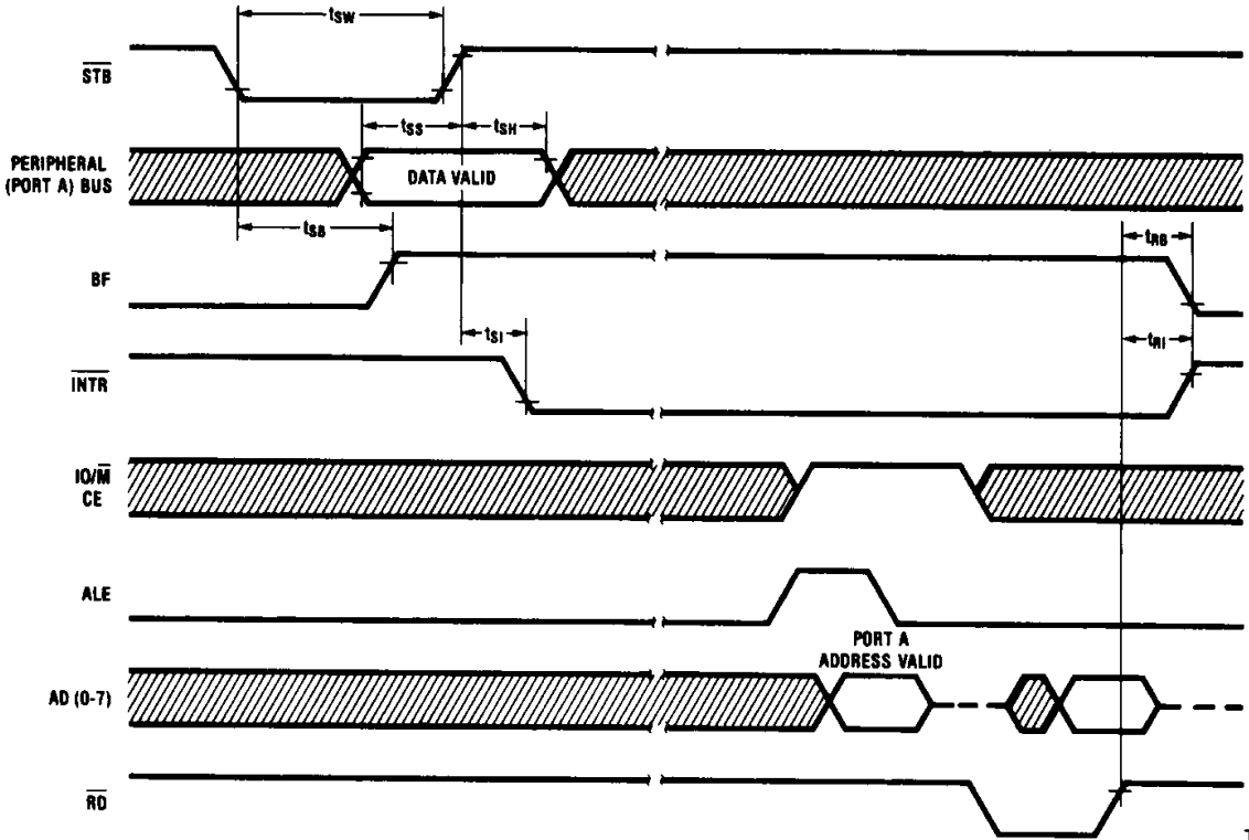
Strobed Mode Input
