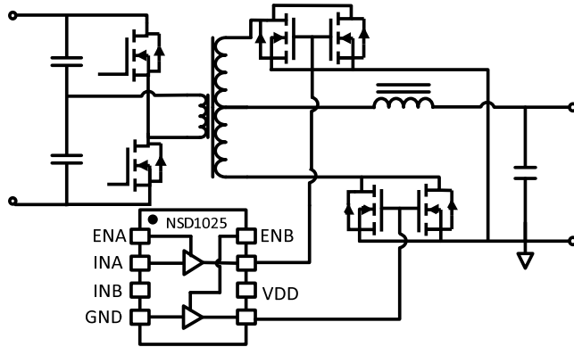
Figure 7.1 Synchronous Rectifier
