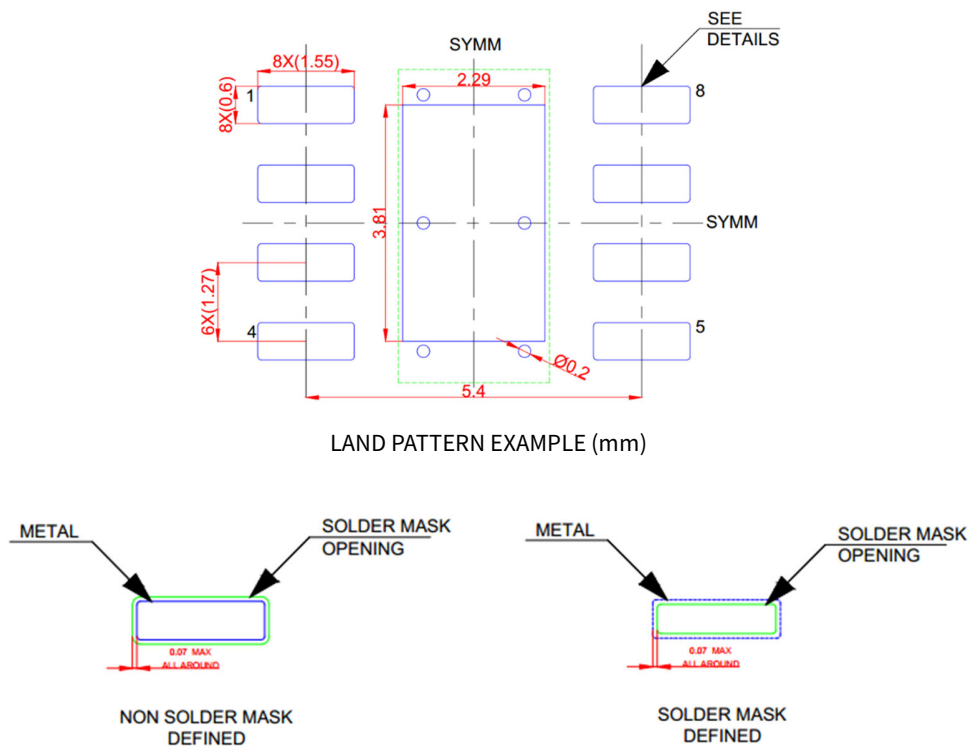
Figure 8.2 HSOP8 Solder Mask Detail
