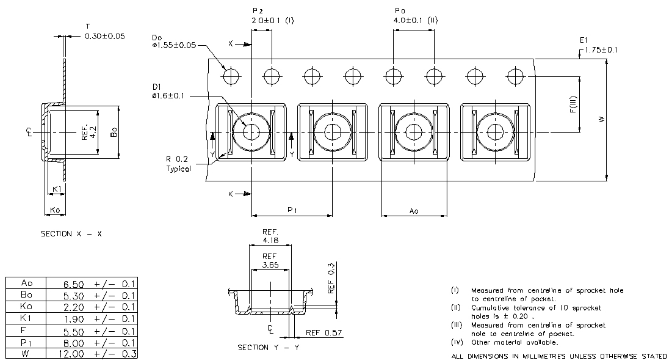
Figure 11.3 Reel information of HSOP8
