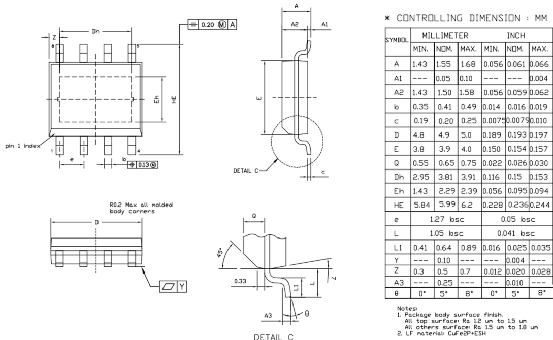
Figure 8.1 HSOP8 Package Shape and Dimension
