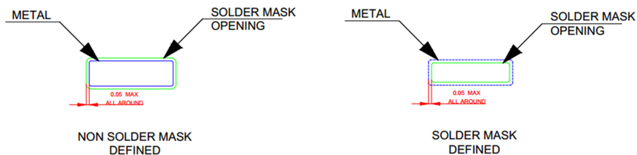
Figure 8.4 HMSOP8 Solder Mask Detail
