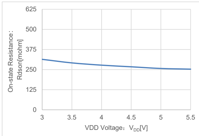
Figure 6.1. On-state Resistance vs VDD Voltage
