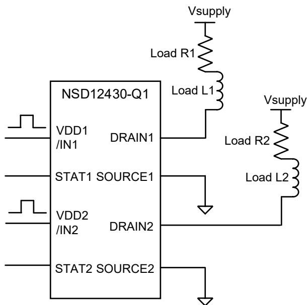
Figure 0.1 NSD12430-Q1 Typical Application
