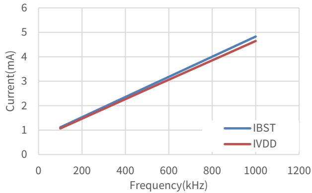
Figure 6.1 Operating Current (I_VDD, I_BST) vs. Frequency (VDD = VBST=12 V, SW = PGND, 330pF load)
