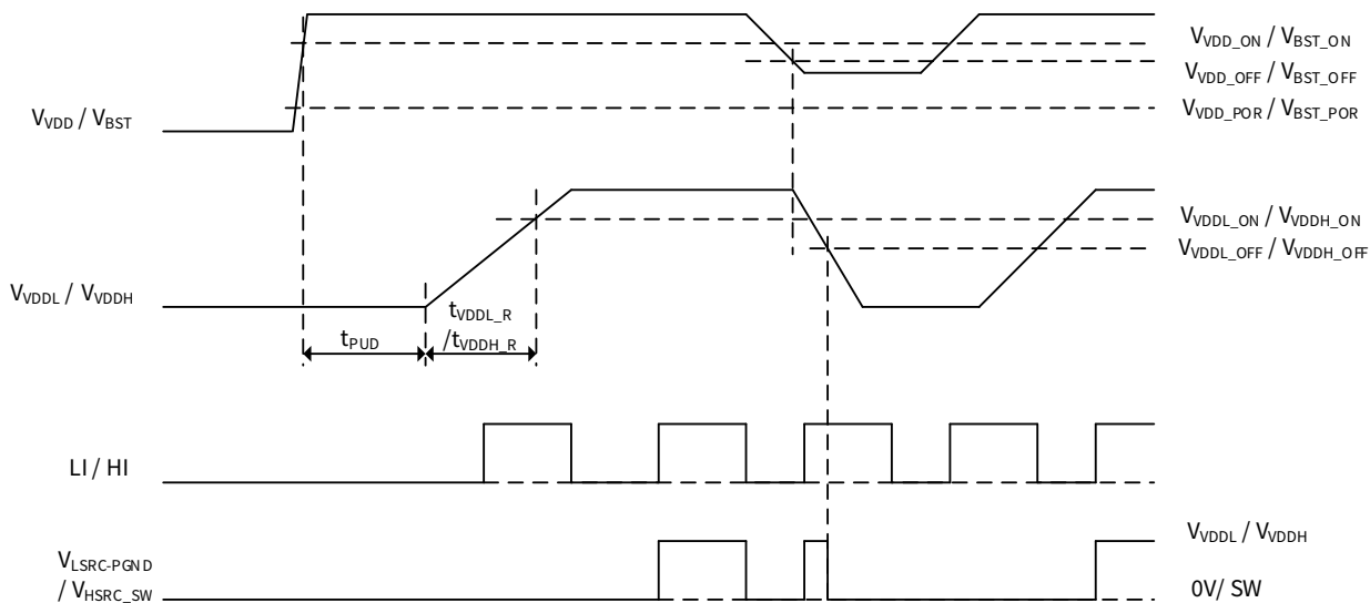
Figure 7.1 UVLO Diagram
