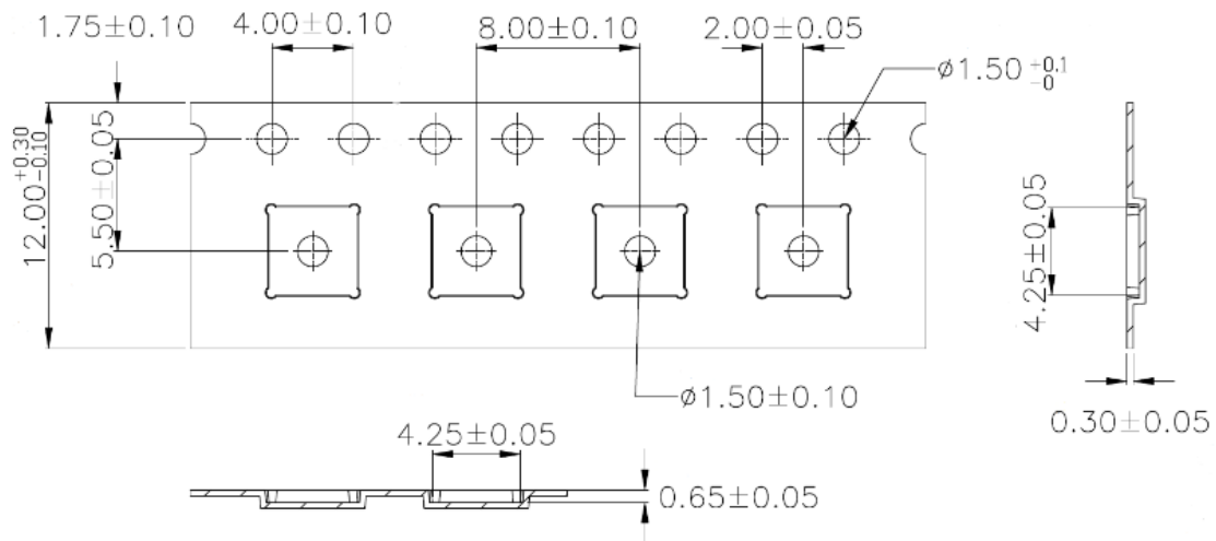
Figure. 11.2 Reel Information
