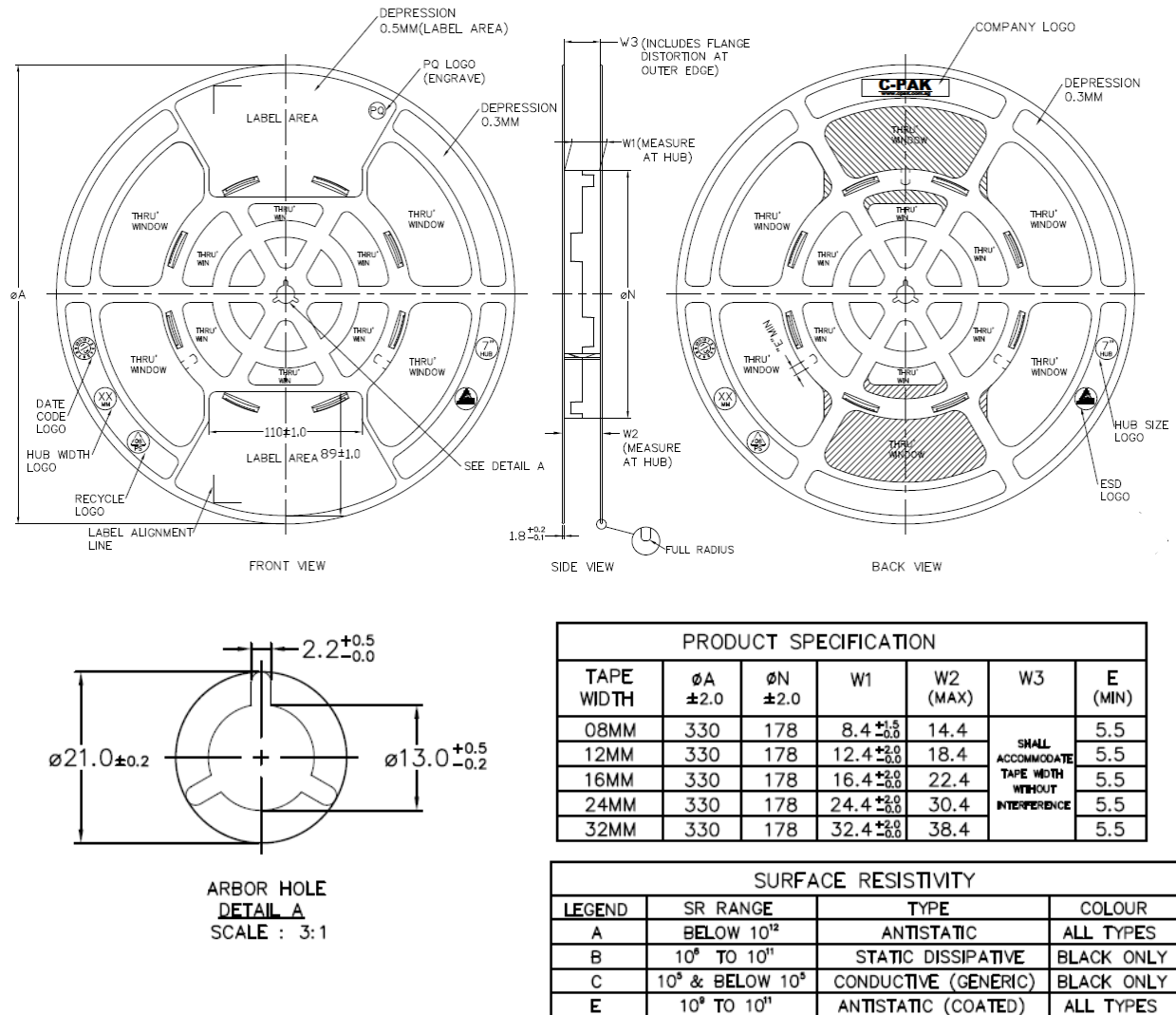
Figure. 11.1 Tape Information
