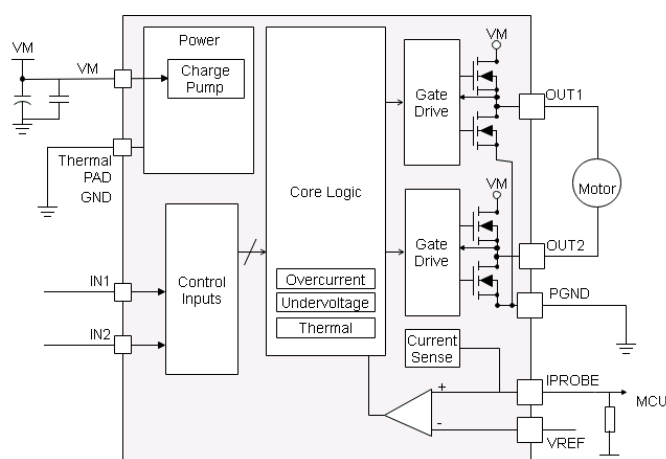
Figure 1. NSD7310A Block Diagram
