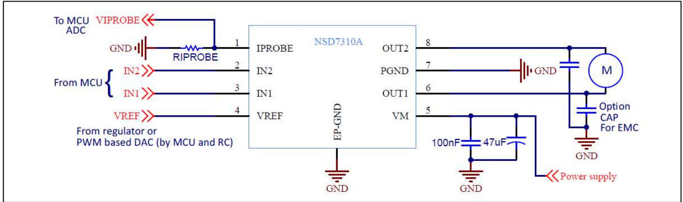
Figure 4. Typical application connection
