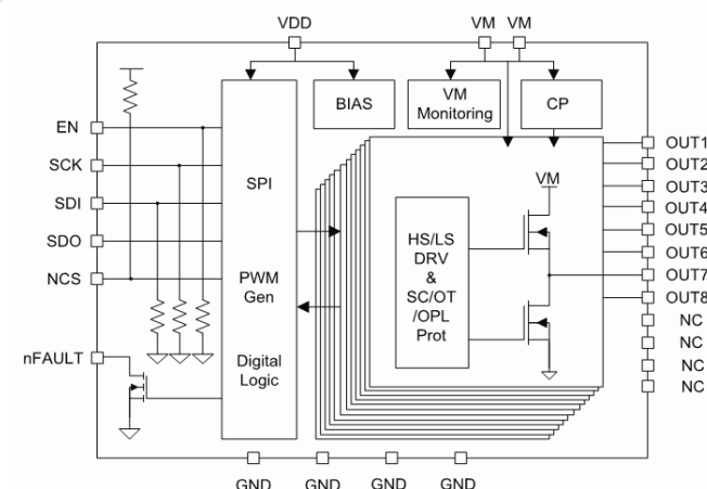
Figure 1. NSD8308 Block Diagram
