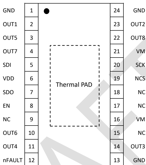
Figure 2. NSD8308 Pinout
