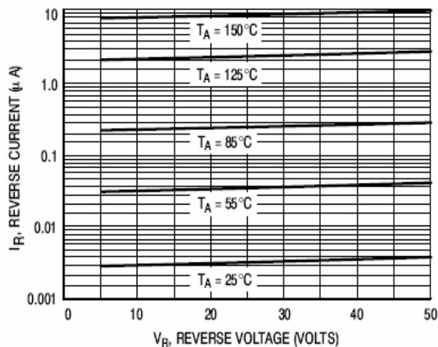
Figure 2. Leakage Current
