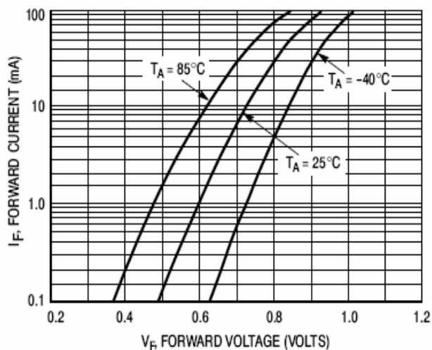
Figure 1. Forward Voltage
