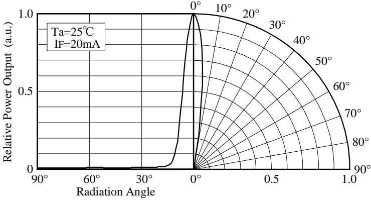
■ Directivity (NSHU590A)
