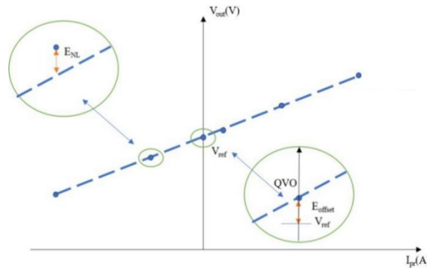
Figure 5.3 NSM2011 sensitivity and error
