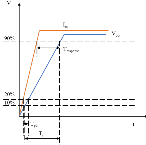
Figure 5.2 NSM2011 response time
