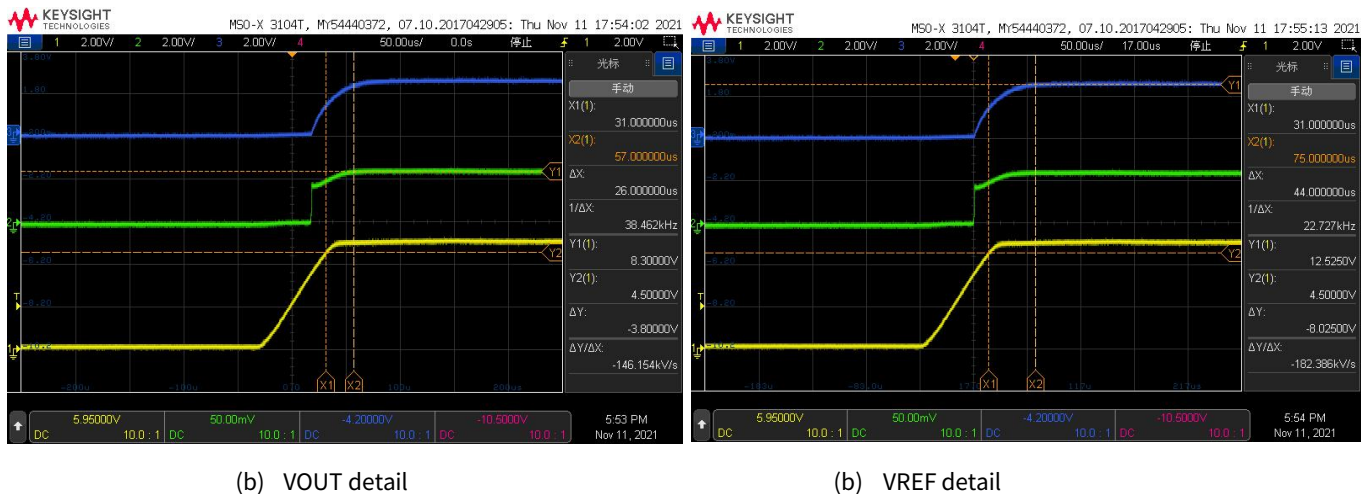
Figure 4.2 NSM2013 Power-on time wave (10kΩ Resistance connected between VOUT and VREF)
