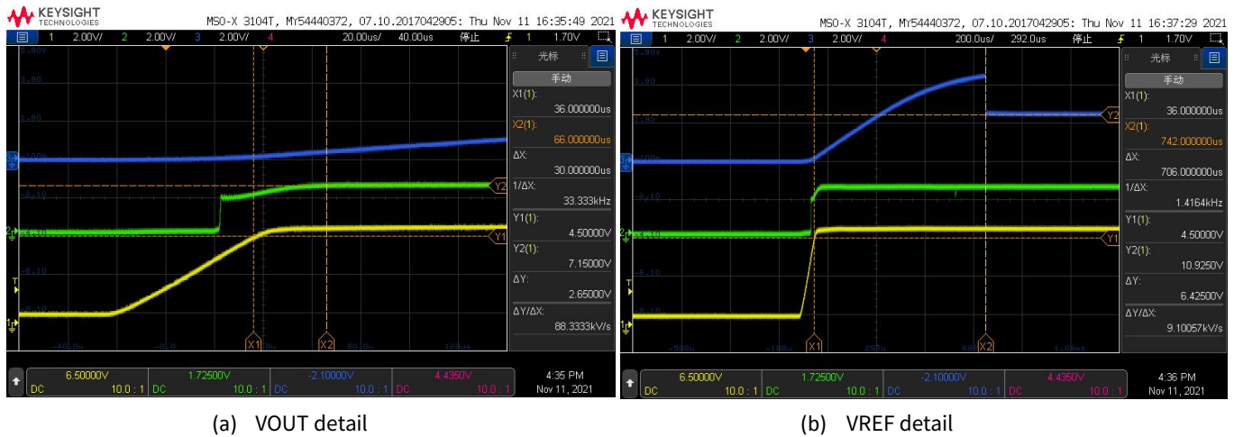
Figure 4.1 NSM2013 Power-on time wave
