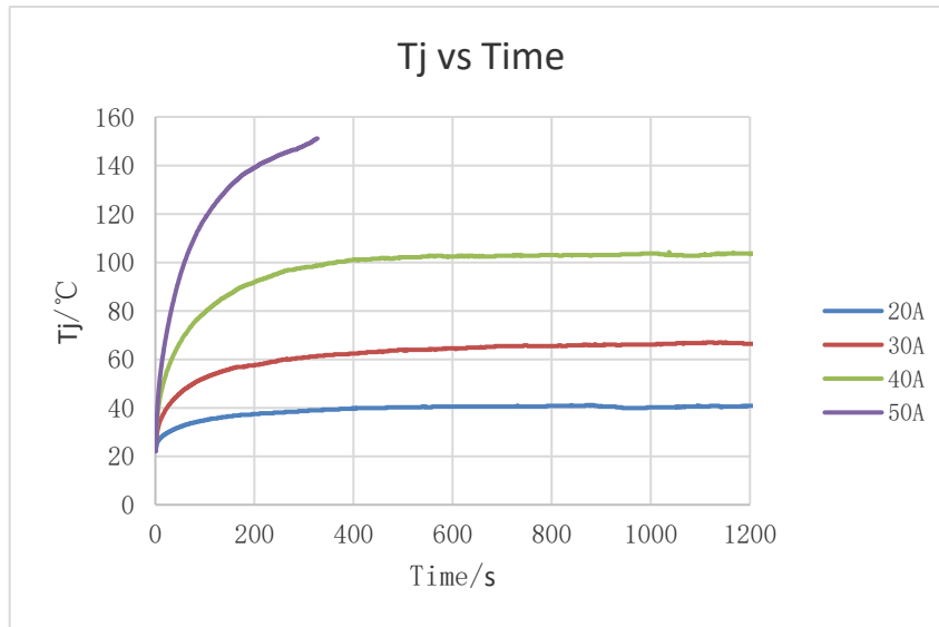
Figure 7.3 NSM2017 Junction temperature vs. Different continues current
