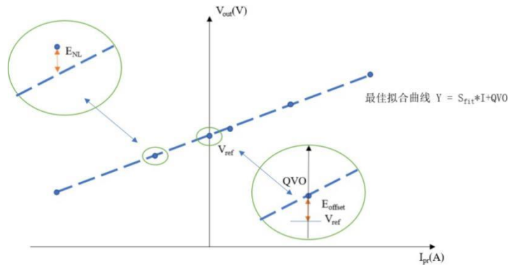
Figure 6.4 NSM2017 Sensitivity and error
