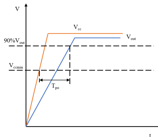
Figure 6.2 NSM2017 Power-on time
