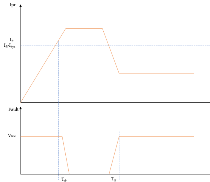
Figure 6.1 NSM2017 Overcurrent Performance
