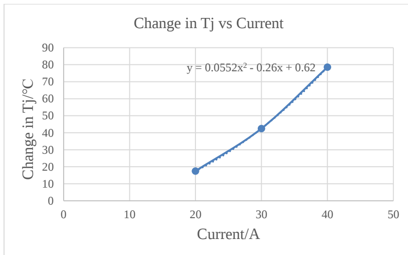
Figure 7.4 NSM2017 Estimation function of junction temperature at different currents (PCB is in the worst case)
