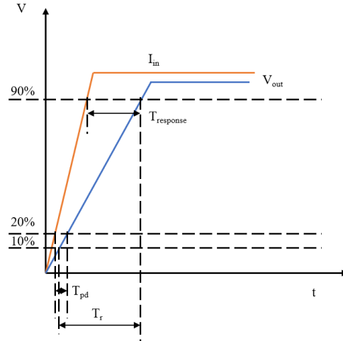
Figure 6.3 NSM2017 response time
