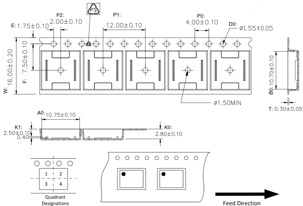
Figure 10.1 Tape and Reel Information of SOW16
