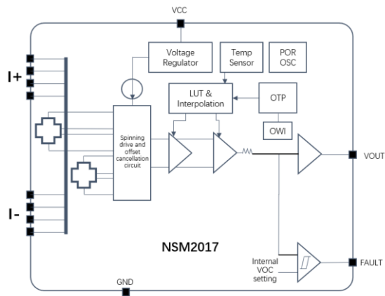
Figure 1. NSM2017 Block Diagram
