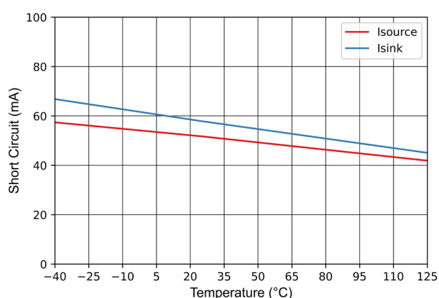
Figure 7-34 Short-Circuit vs Temperature
