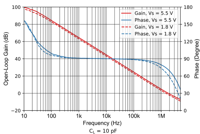
Figure 7-12 Open Loop Gain vs Frequency
