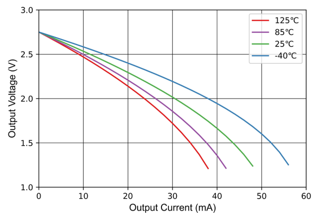
Figure 7-36 Output Voltage Swing vs Output Sourcing Current
