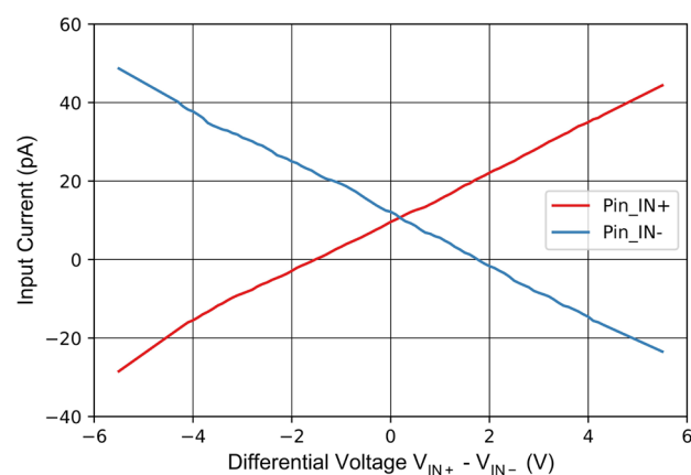
Figure 7-33 Input Current vs Differential Voltage ( V_{IN+} - V_{IN-} )
