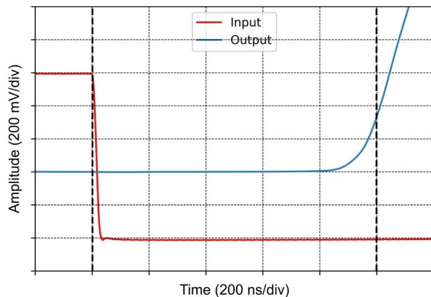
Figure 7-26 Negative Overload Recovery ( G = -10 )
