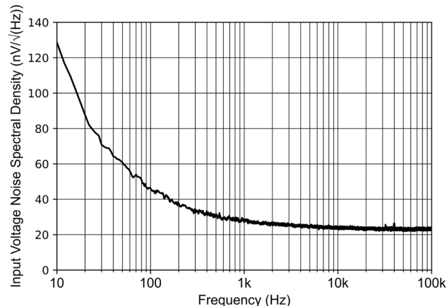
Figure 7-28 Input Voltage Noise Spectral Density
