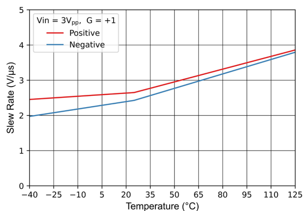
Figure 7-22 Slew Rate vs Temperature
