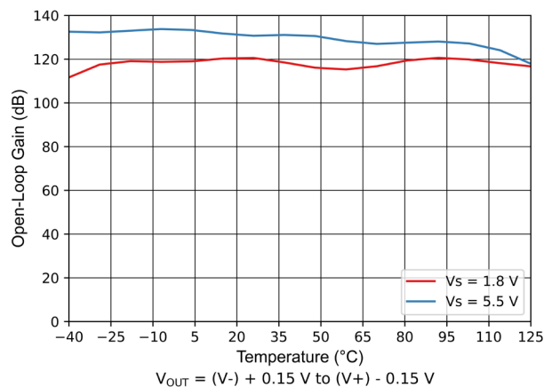
Figure 7-11 Open-Loop Gain vs Temperature
