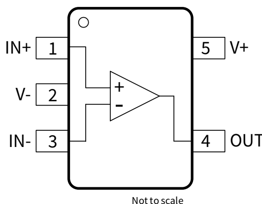
Figure 1-2 NSOPA8011-Q1 5-Pin SC70 Package Top View
