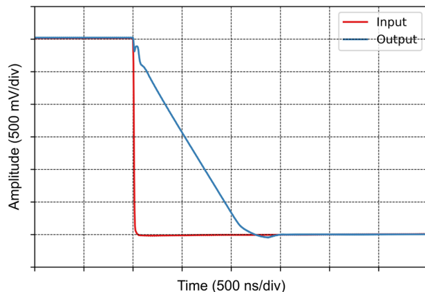
Figure 7-20 Large-Signal Step Response (Falling)
