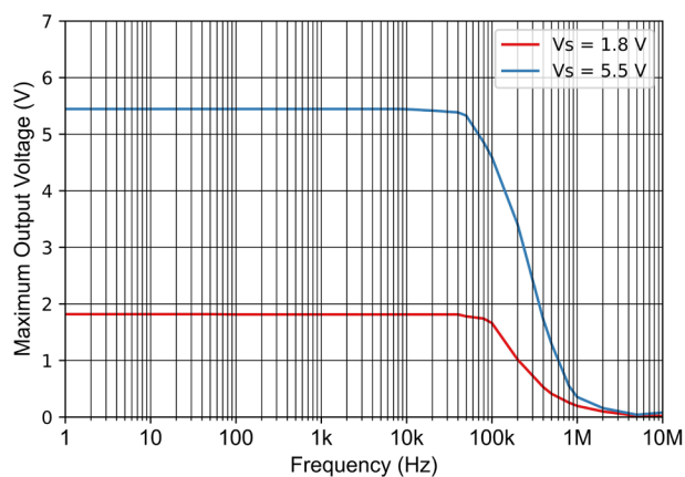
Figure 7-18 Maximum Output Voltage vs Frequency
