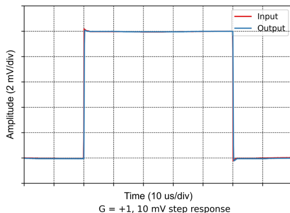
Figure 7-24 Small-Signal Step Response
