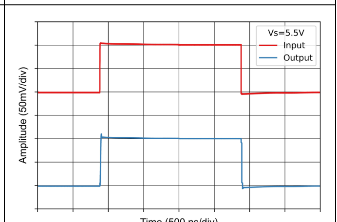
Figure 7-24 Small-Signal Step Response
