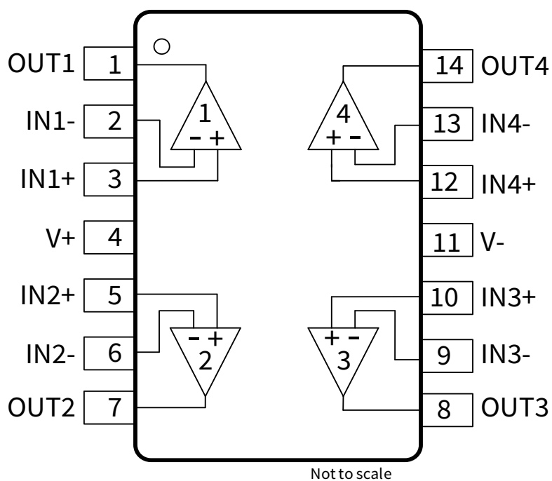
Figure 1-4 NSOPA8054-Q1 14-Pin SOP and TSSOP Package Top View
