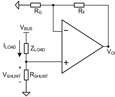
Figure 9-3 NSOPA805x-Q1 in a Low-Side, Current-Sensing Application
