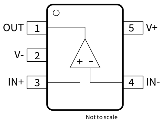
Figure 1-1 NSOPA8051-Q1 5-Pin SOT23 Package Top View
