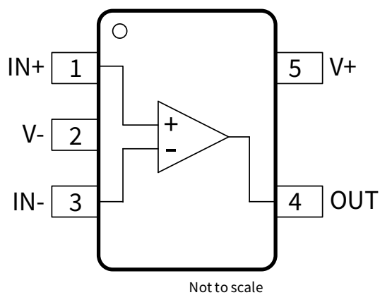
Figure 1-2 NSOPA8051-Q1 5-Pin SC70 Package Top View
