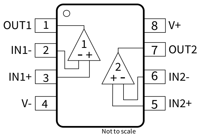
Figure 1-3 NSOPA8052-Q1 8-Pin SOP and MSOP Package Top View
