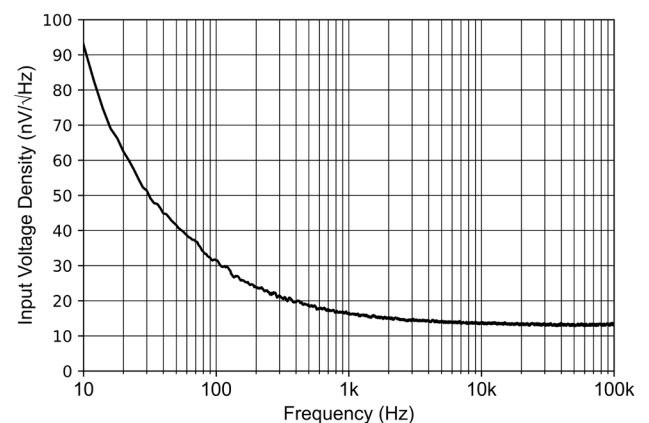
Figure 7-28 Input Voltage Noise Spectral Density
