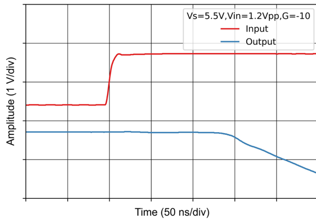
Figure 7-25 Positive Overload Recovery ( G = -10 )
