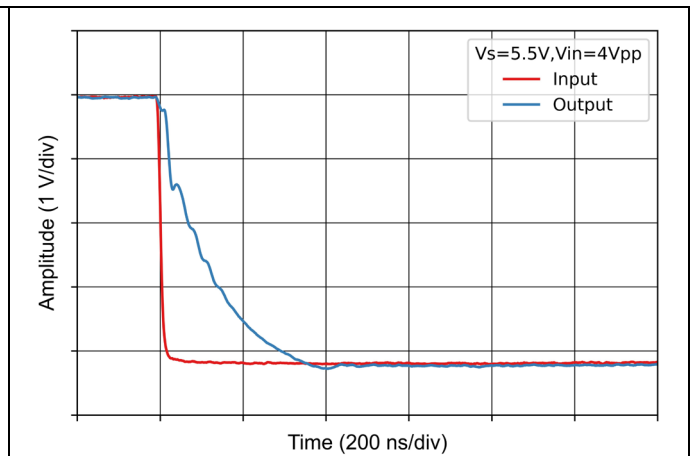
Figure 7-20 Large-Signal Step Response (Falling)
