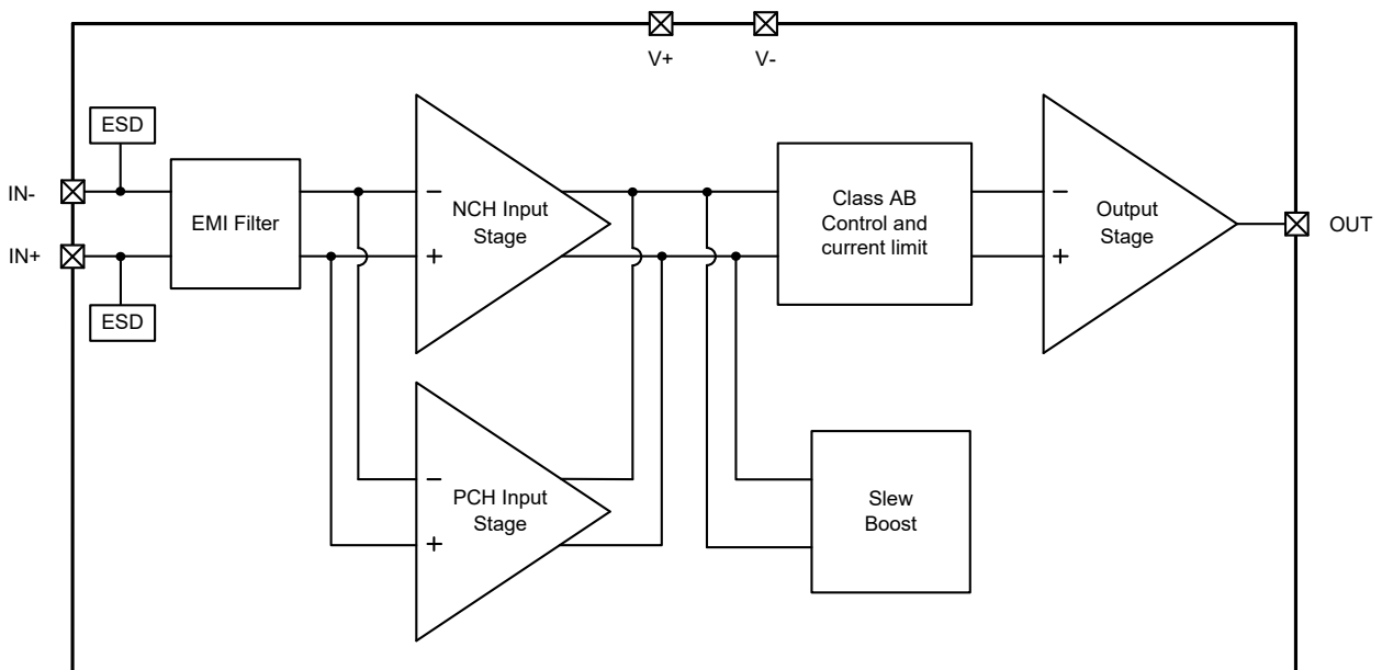
Figure 8-1 NSOPA805x-Q1 Functional block Diagram (One channel is shown)
