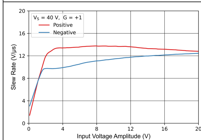
Figure 7-21 Slew Rate vs Input Voltage Amplitude
