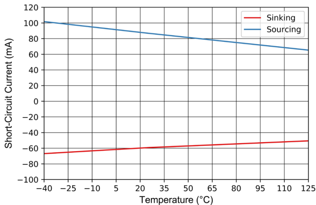
Figure 7-35 Short-Circuit vs Temperature
