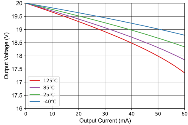
Figure 7-34 Output Voltage Swing vs Output Sourcing Current
