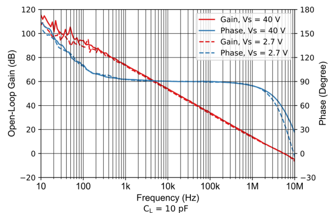
Figure 7-12 Open Loop Gain vs Frequency
