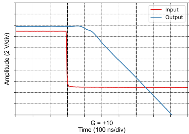
Figure 7-26 Negative Overload Recovery
