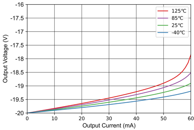
Figure 7-33 Output Voltage Swing vs Output Sinking Current
