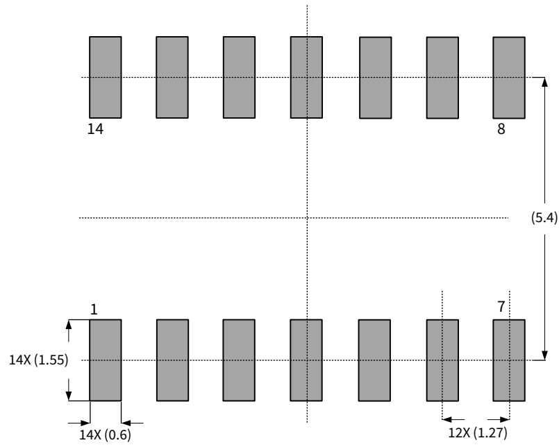
SOP14
