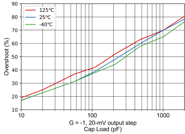
Figure 7-32 Small-Signal Overshoot vs Capacitive Load
