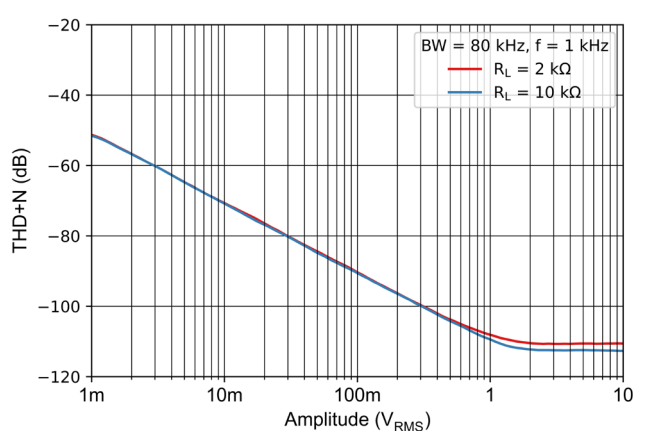
Figure 7-30 THD+N vs Output Amplitude
