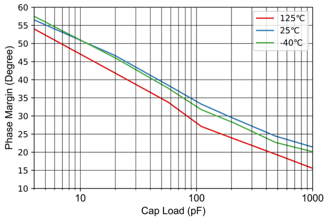
Figure 7-31 Phase Margin vs Capacitive Load
