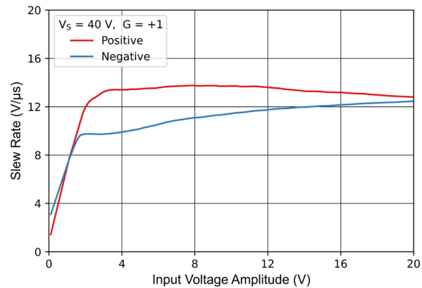
Figure 8-5 Slew-Rate vs Input Voltage Amplitude
