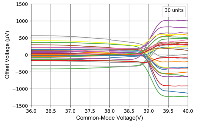
Figure 7-4 Offset Voltage vs Common-Mode Voltage (Transition Area)
