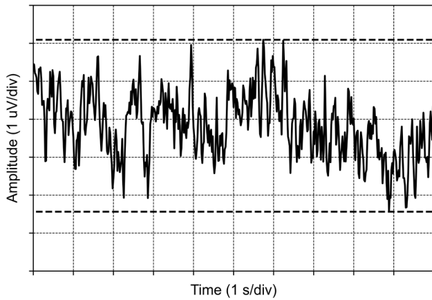
Figure 7-27 0.1-Hz to 10-Hz Noise
