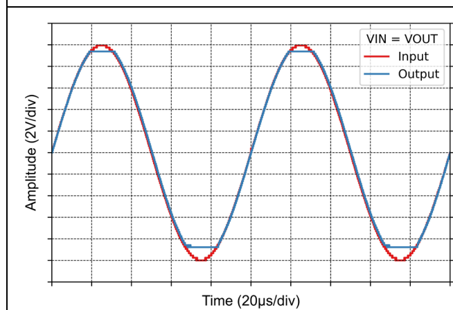
Figure 7-23 No Phase Reversal
