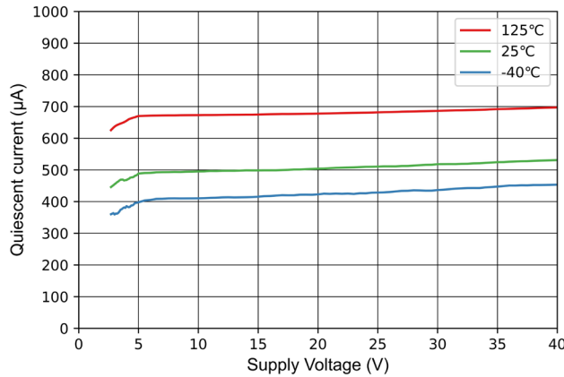
Figure 7-13 Quiescent Current vs Supply Voltage ( V_{CM} = V_- )
