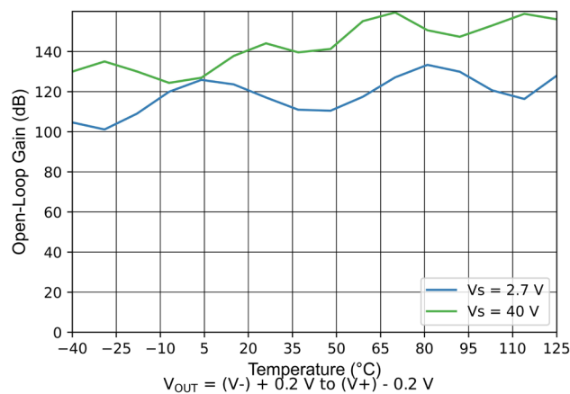
Figure 7-11 Open-Loop Voltage Gain vs Temperature
