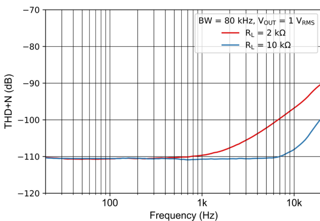
Figure 7-29 THD+N Ratio vs Frequency
