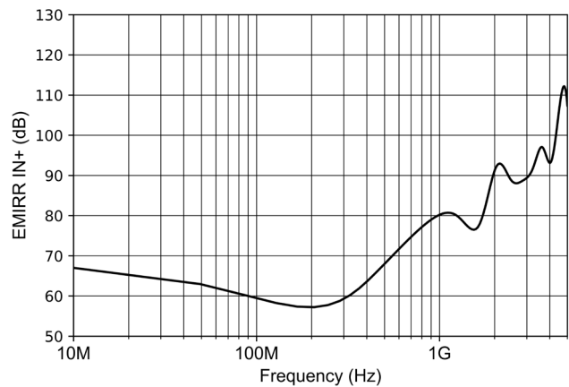
Figure 7-36 EMIRR vs Frequency
