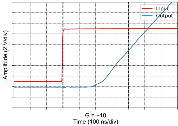
Figure 7-25 Positive Overload Recovery
