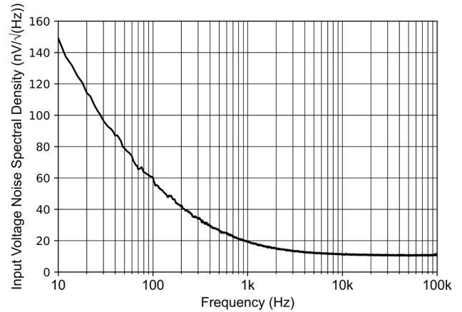
Figure 7-28 Input Voltage Noise Spectral Density
