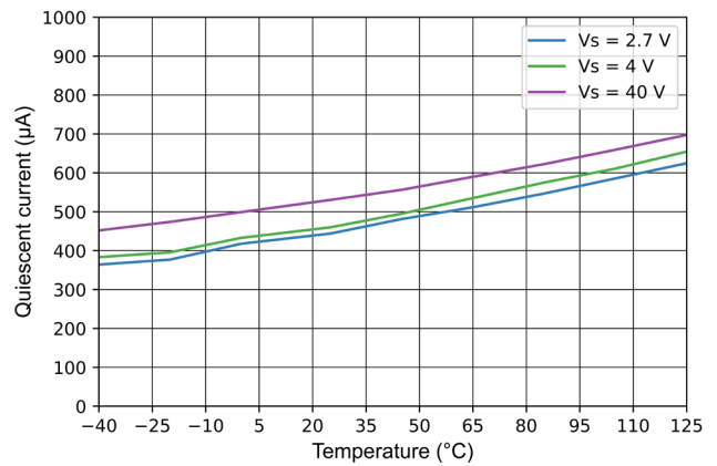
Figure 7-14 Quiescent Current vs Temperature
