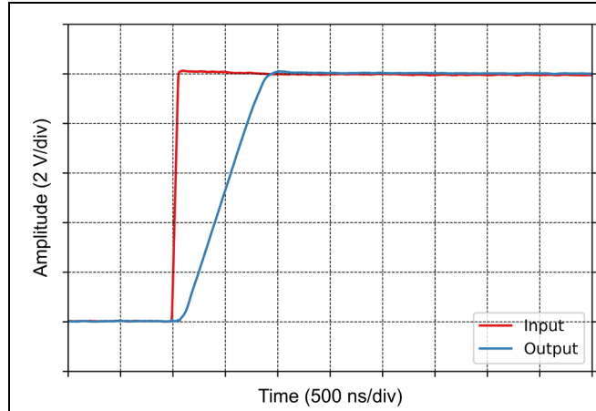
Figure 7-19 Large-Signal Step Response (Rising)
