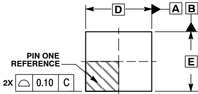
2X 0.10 C TOP VIEW
