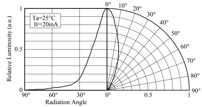
■ Directivity (NSPG310A)
