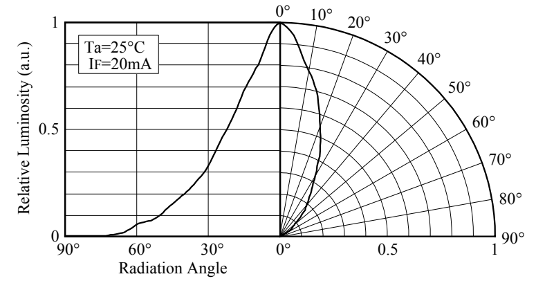
■ Directivity (NSPG320BS)
