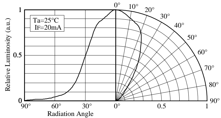
■ Directivity (NSPW310BS)
