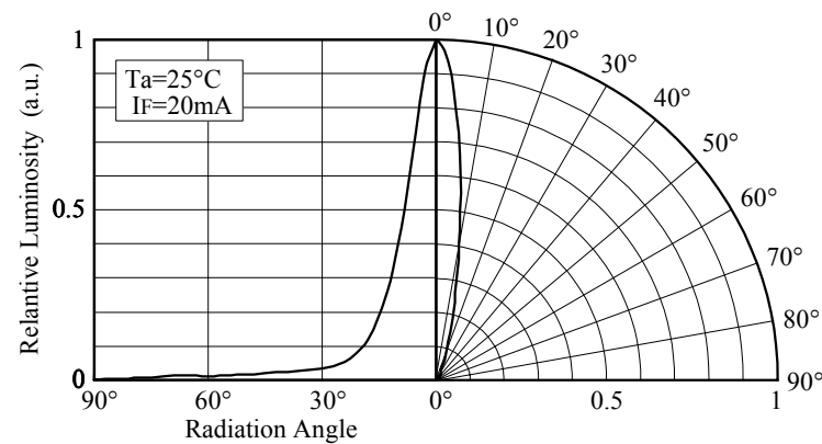
■ Directivity (NSPY500S)
