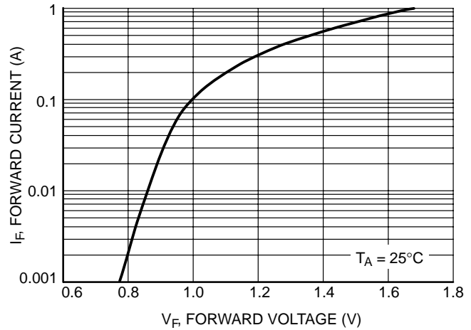
Figure 6. Forward Voltage
