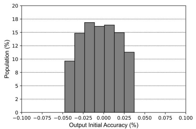
Figure 7.6 Accuracy Distribution
