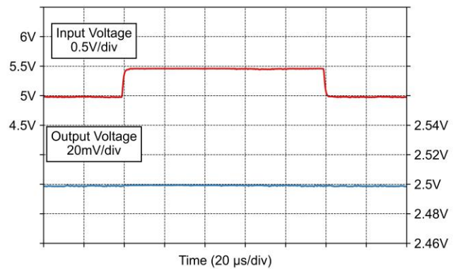
Figure 7.12 Line Transient Response ( C_L=1\mu F )
