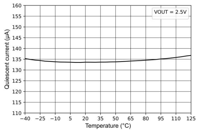
Figure 7.4 Quiescent Current vs Temperature
