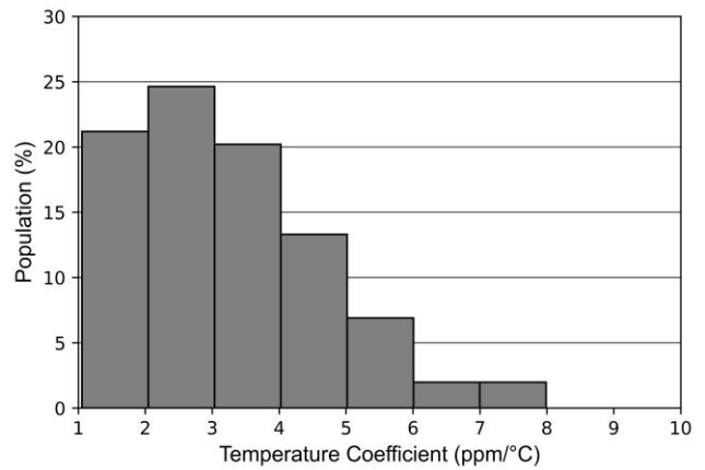
Figure 7.2 Temperature Drift Histogram
