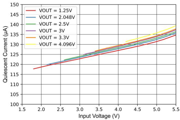
Figure 7.3 Quiescent Current vs Input Voltage
