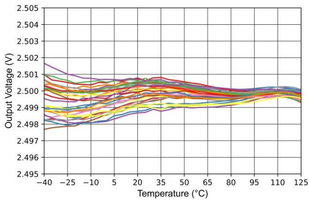
Figure 7.1 Output Voltage vs Temperature
