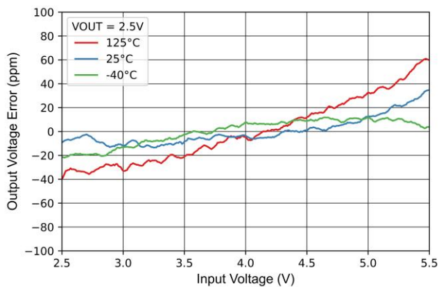
Figure 7.5 Output Voltage Error vs Input Voltage
