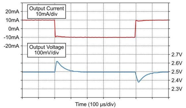
Figure 7.16 Load Transient Response \pm 10\text{mA} ( C_L=1\mu\text{F} )
