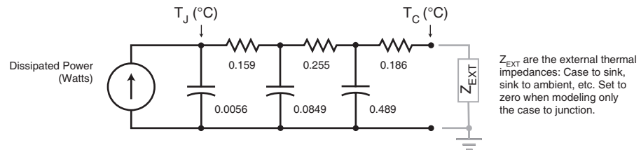
Fig.1b Transient thermal impedance model
