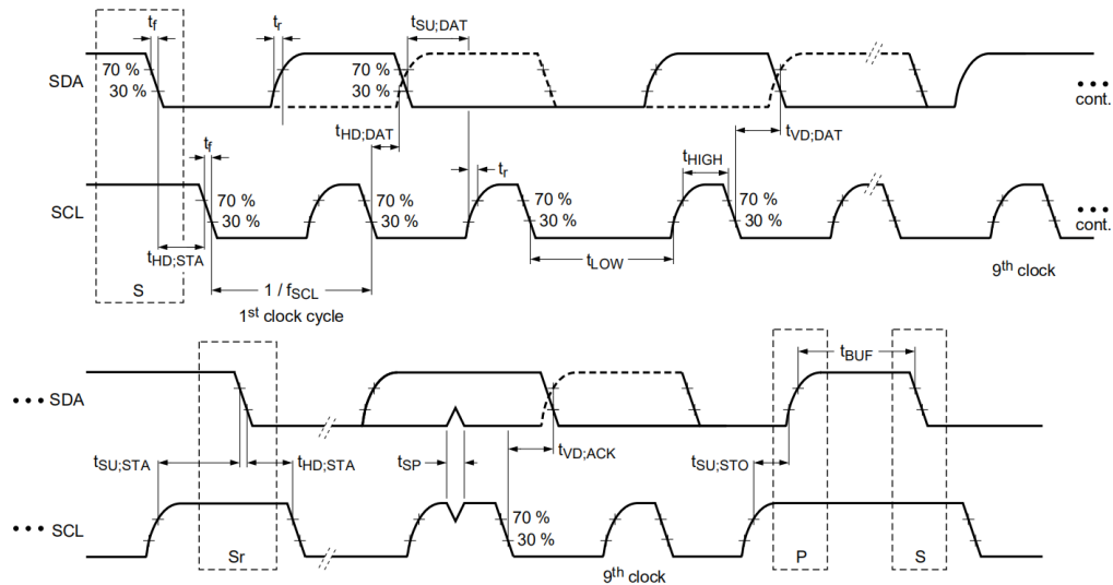
Figure 3.1 I 2 C Timing Diagram
