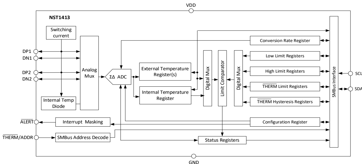
Figure 4.1 NST1413 Functional Block Diagram
