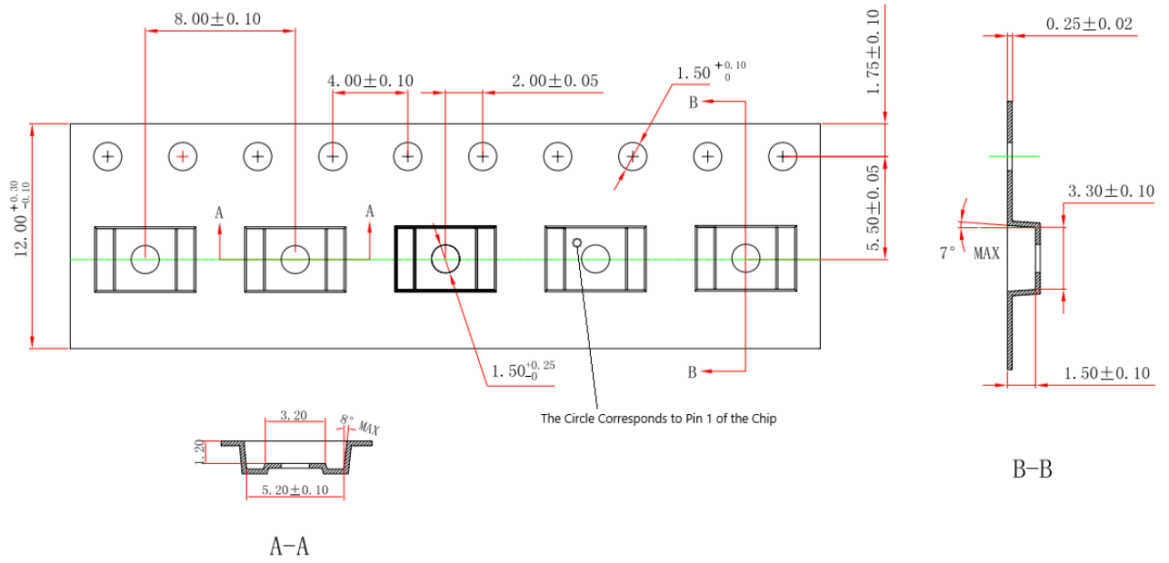
MSOP (10) TAPE Information (in mm)
