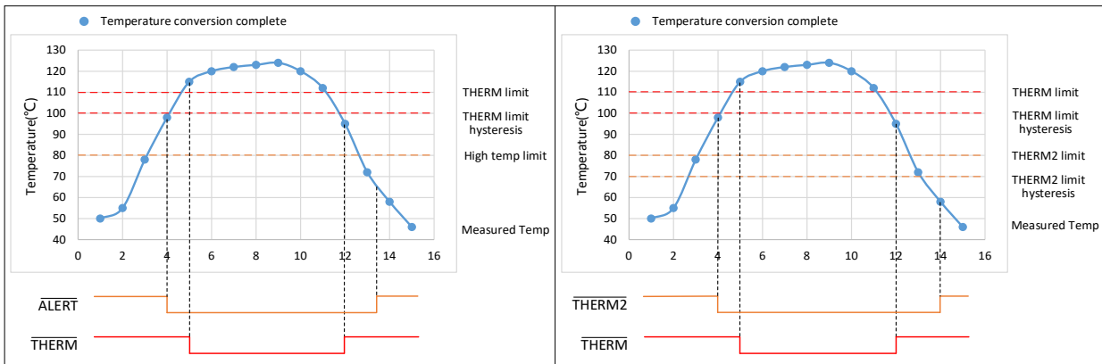
Figure 4.4 ALERT and THERM interrupt operation Figure 4.5 THERM and THERM2 interrupt operation
