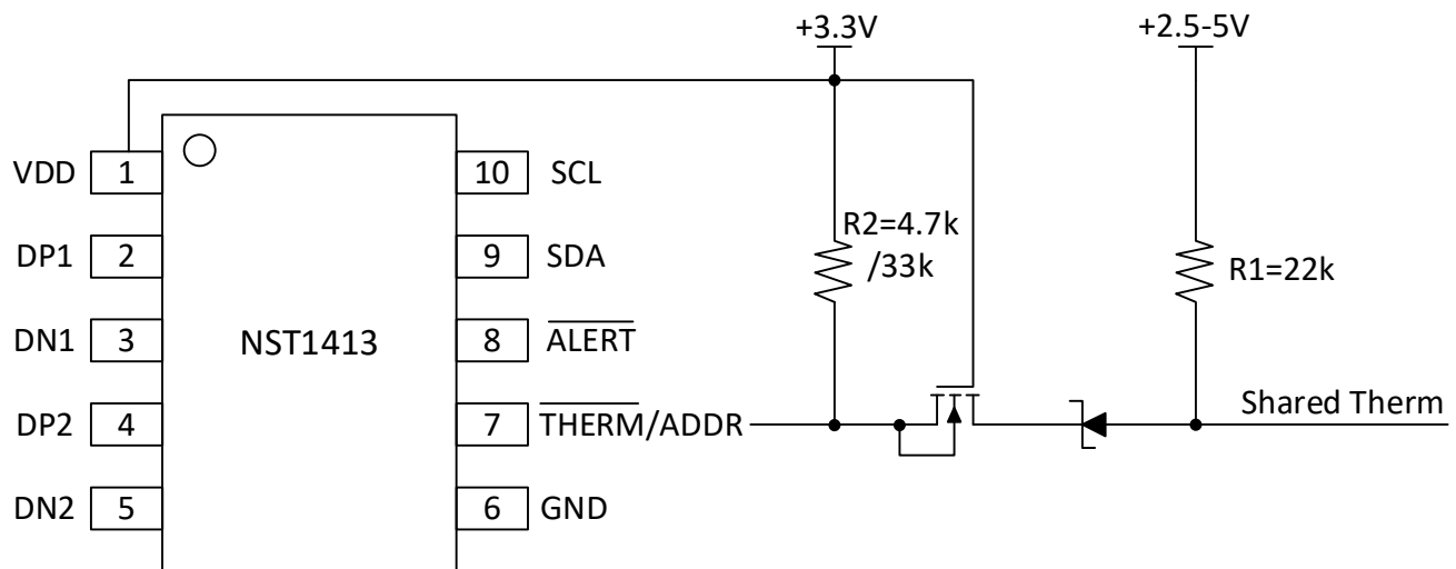
Figure 4.8. Isolating THERM Pin
