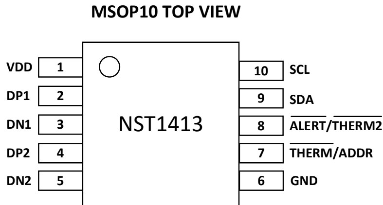
Figure 1.1 NST1413 Package
