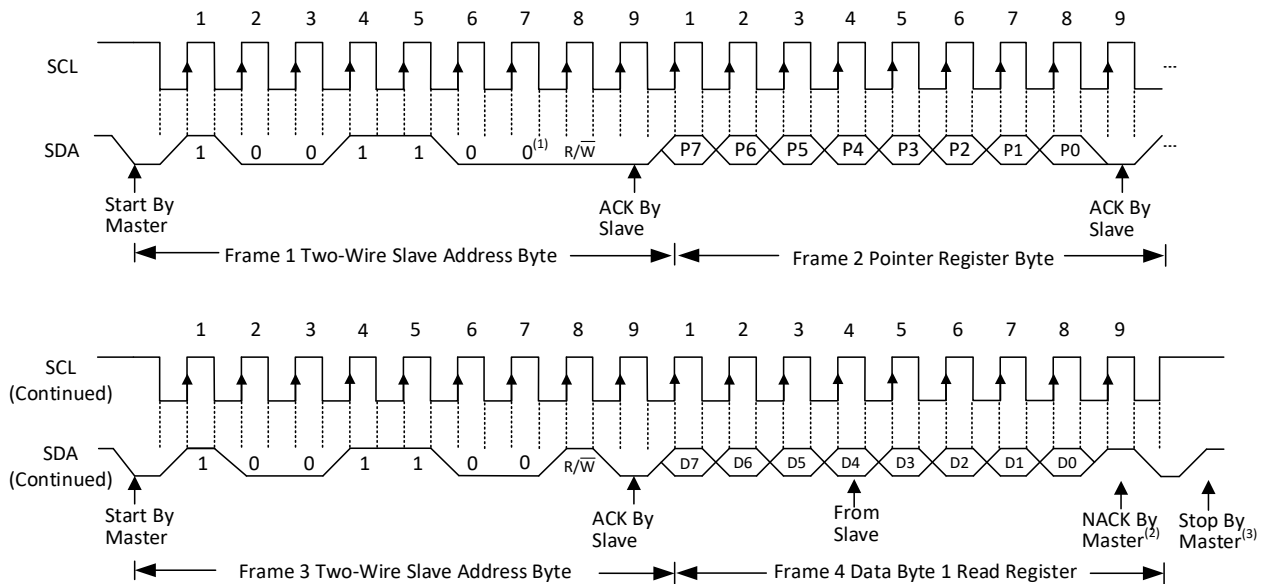
Figure 4.6. Two-Wire Timing Diagram for the NST1413 Write Word Format
