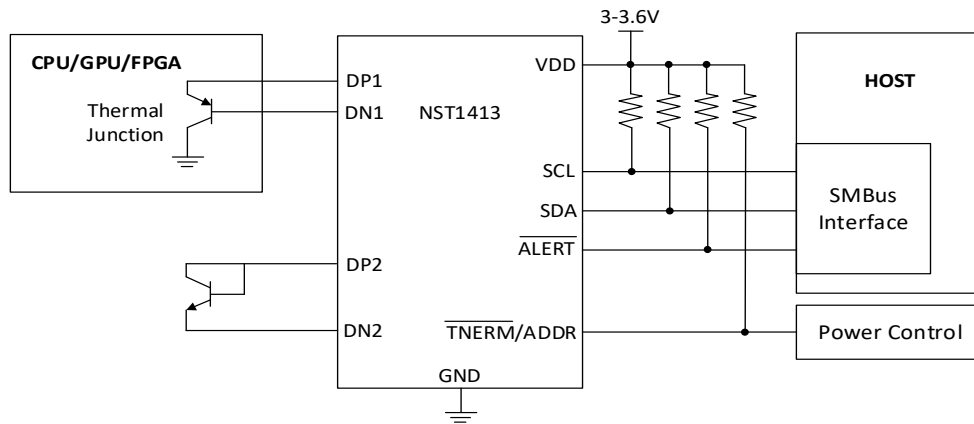
Figure 6.1. NST1413 Basic Connections Using a Discrete Remote Transistor
