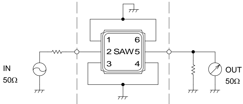
Fig.1 Measuring circuit
