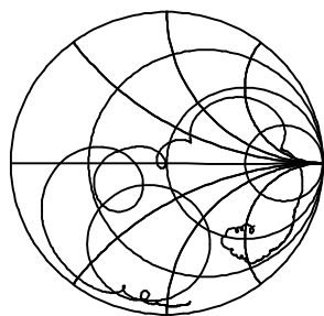
S11
