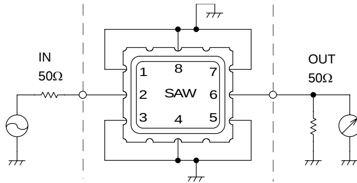
Fig.1 Measuring circuit
