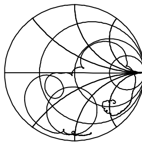
S22
