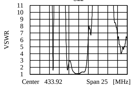
S22
