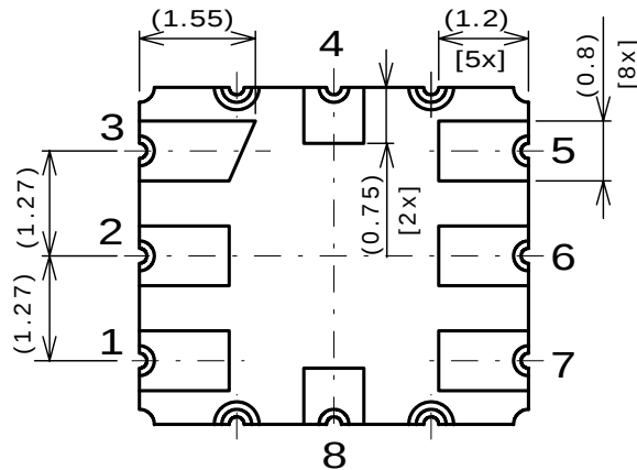
Fig.2 Package dimensions (in mm)
