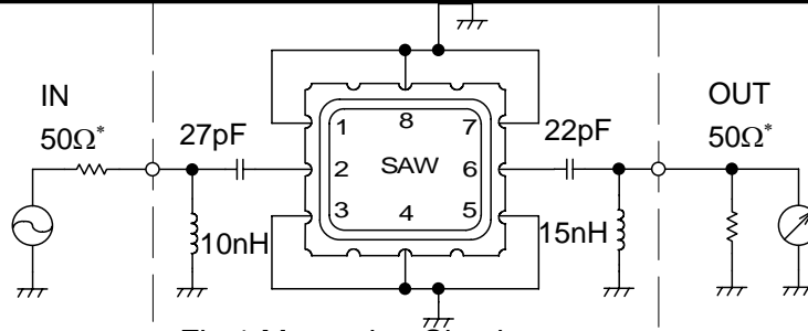
Fig.1 Measuring Circuit
