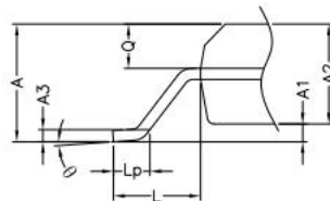
Figure 9.1 SOW8 Package Shape and Dimension in millimeters
